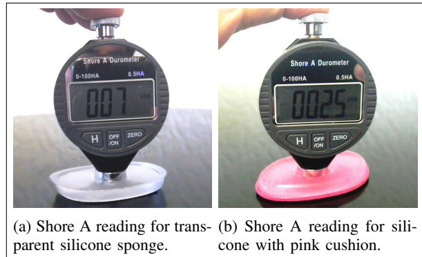
Fig. 2: Shore A measurements of silicone sponges.
